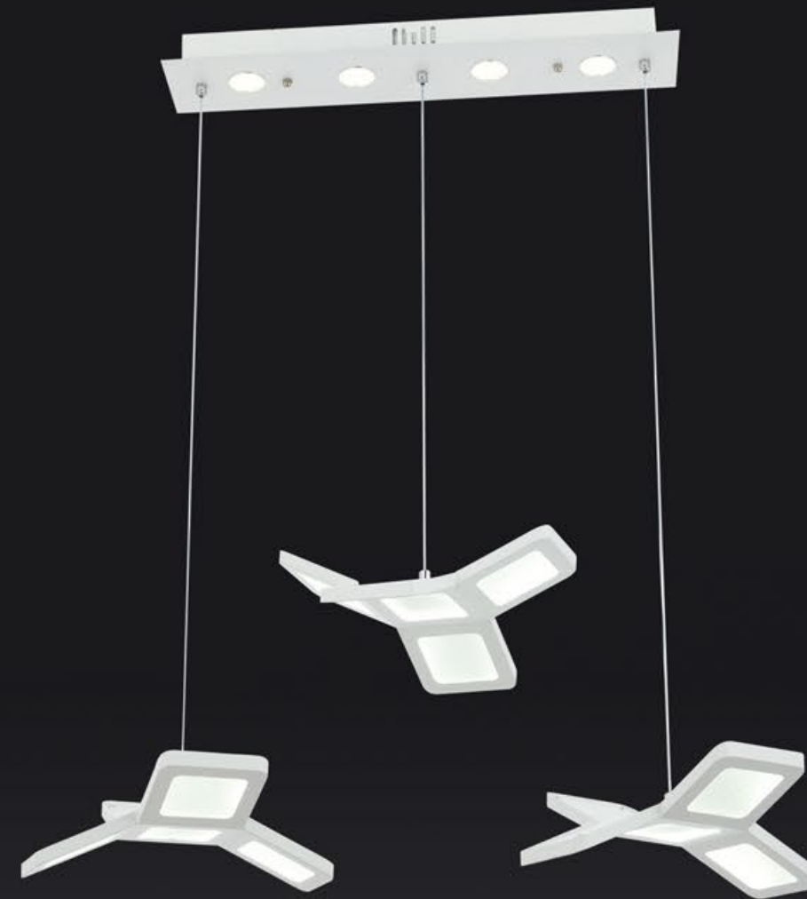
1012-4 W:75x30 H:100 Tepsi: Power LED 4x3W Kol: Power LED 3x15W
